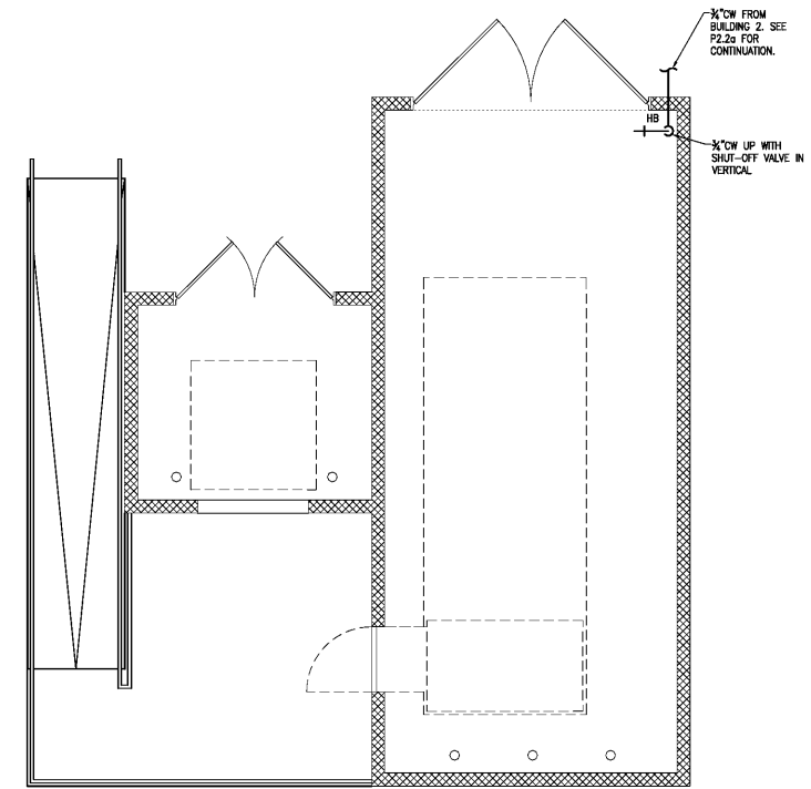
3 Trash Enclosure - Water Scale: 1/4" = 1'-0"
