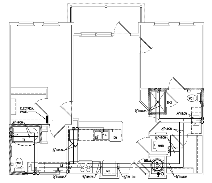
④ Unit B1 - Typical Floor - Water Scale: 1/4" = 1'-0" B1-ALT1 & B1-ALT2 ARE SIMILAR
