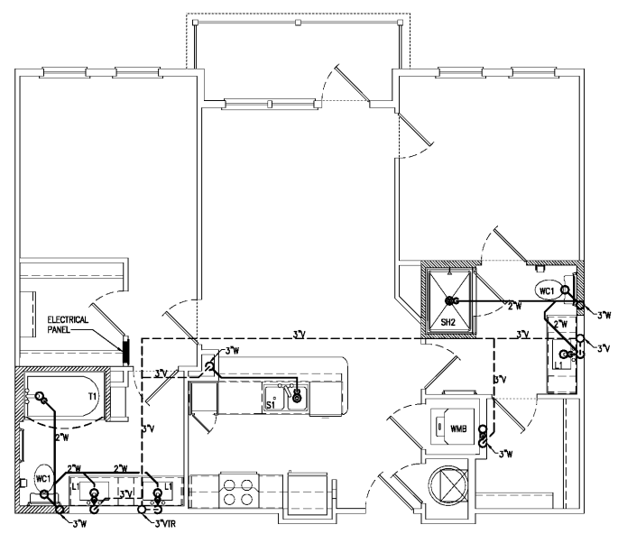
① Unit B1 - Top Floor - S,W,&V Scale: 1/4" = 1'-0" B1-ALT1 & B1-ALT2 ARE SIMILAR
