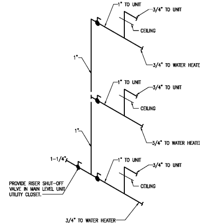
1 WATER RISER DIAGRAM - ONE BATHROOM NO SCALE
