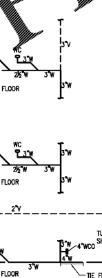
18 S.W.&V RISER DIAGRAM NO SCALE
