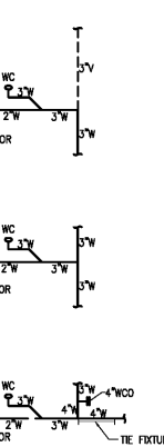
22 S.W.&V RISER DIAGRAM NO SCALE
