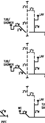
19 S.W.&V RISER DIAGRAM NO SCALE
