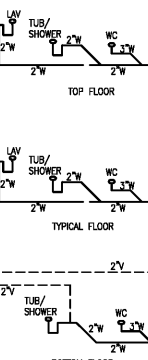
14 S.W.&V RISER DIAGRAM NO SCALE
