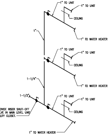
2 WATER RISER DIAGRAM - TWO BATHROOM NO SCALE
