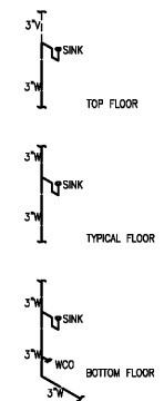
6 S.W.&V RISER DIAGRAM NO SCALE
