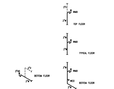
5 S.W.&V RISER DIAGRAM NO SCALE
