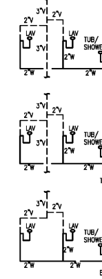
21 S.W.&V RISER DIAGRAM NO SCALE
