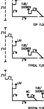
12 S.W.&V RISER DIAGRAM NO SCALE
