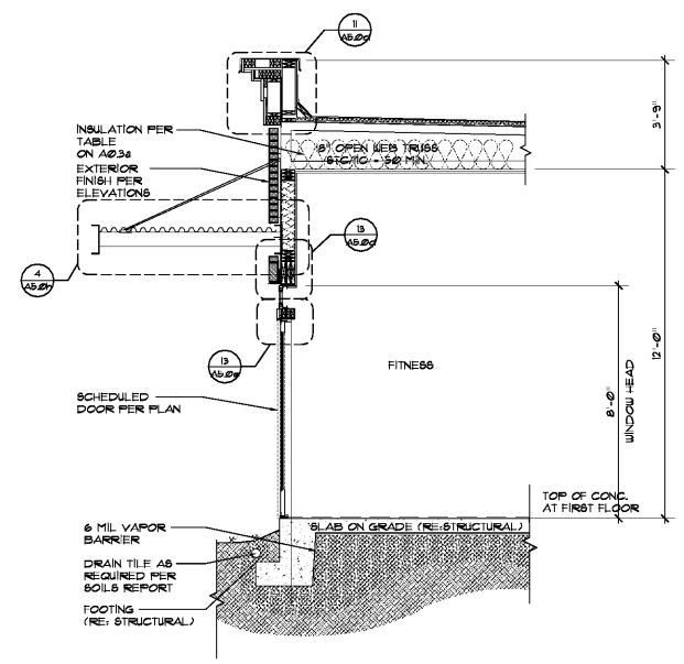
6 Fitness - Wall Section at Main Entrance Scale: 3/8" = 1'-0"
