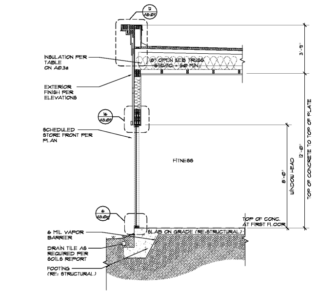
2 Fitness - Wall Section at Panel Siding Scale: 3/8" = 1'-0"
