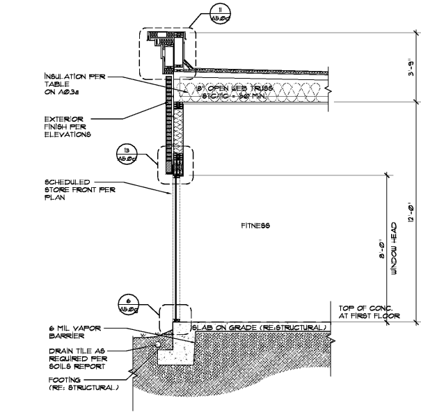
1 Fitness - Wall Section at Brick Scale: 3/8" = 1'-0"
