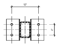
3 SECTION S8.2 1 1/2\"/>
