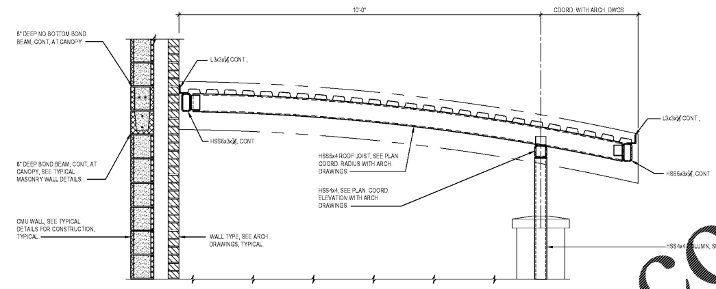
2 SECTION S8.2 3/4\"/>
