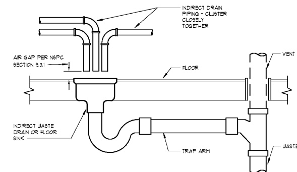
3 INDIRECT WASTE DRAIN DETAIL NOT TO SCALE
