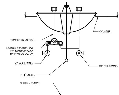
4 LOCAL MIXING VALVE DETAIL NOT TO SCALE
