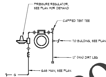
1 GAS METER DETAIL NOT TO SCALE
