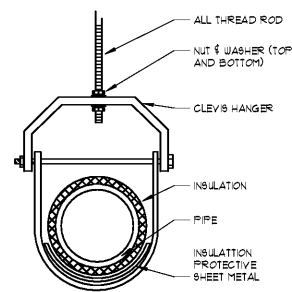
8 TYPICAL CLEVIS HANGER DETAIL NOT TO SCALE
