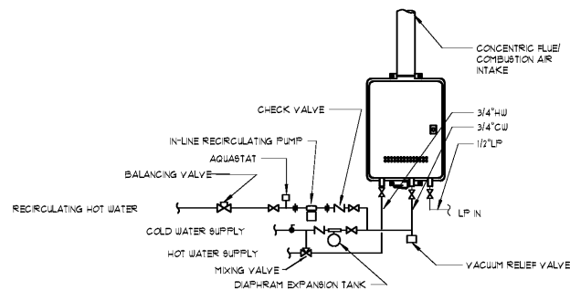
10 TANKLESS WATER HEATER DETAIL NOT TO SCALE
