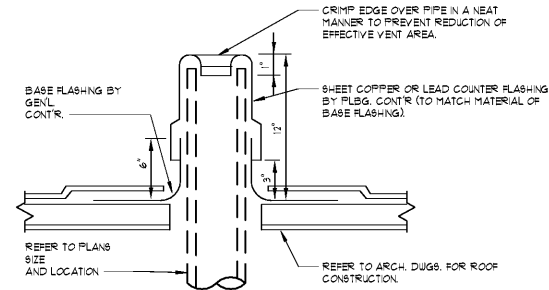
5 PLUMBING VENT THROUGH FLAT ROOF DETAIL NOT TO SCALE
