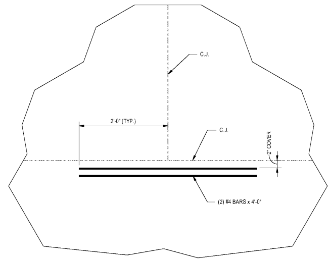
2 CONTROL JOINT T-INTERSECTION DETAIL SCALE: 1" = 1'-0"
