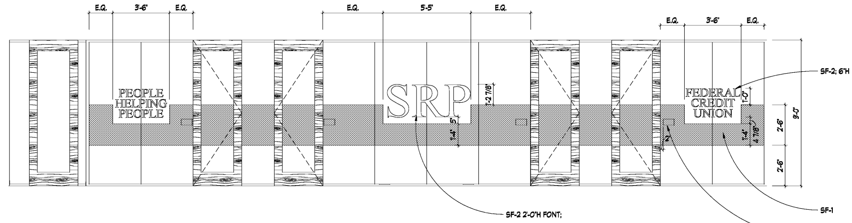
1 SPECIALTY FILM GRAPHIC SCALE: 3/8" = 1'-0"
