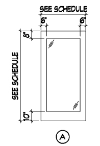
DOOR TYPES SCALE: 1/4" = 1'-0"
