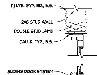
11 HEAD DETAIL SCALE: 1 1/2" = 1'-0"
