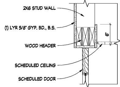
14 HEAD DETAIL SCALE: 1 1/2" = 1'-0"
