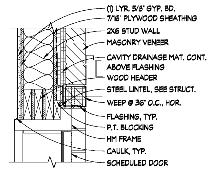
1 HEAD DETAIL SCALE: 1 1/2" = 1'-0"
