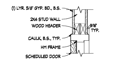
4 HEAD DETAIL SCALE: 1 1/2" = 1'-0"
