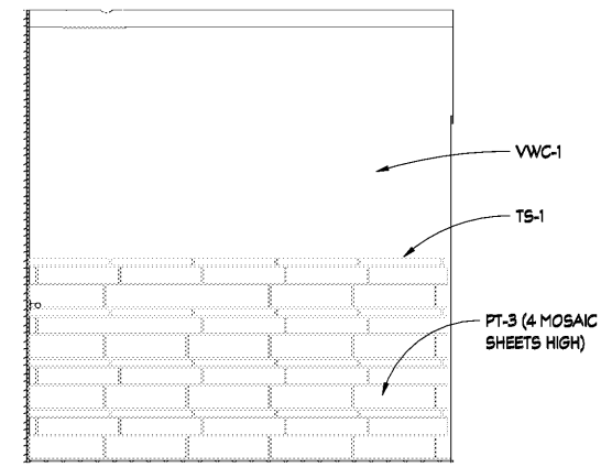
2 TOILET 107 - SOUTH SCALE: 1/2" = 1'-0"
