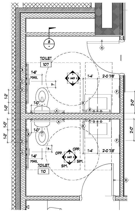
1 TOILET 107 & 110 ENLARGED PLAN A101 SCALE: 1/2" = 1'-0"
