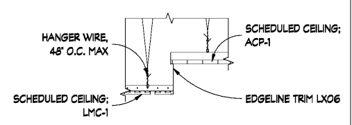
4 SOFFIT @ BREAKROOM A120 SCALE: 1" = 1'-0"
