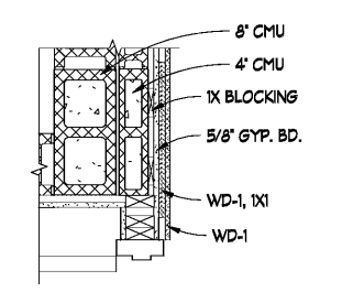
3 FEATURE WALL TILE DETAIL A810 SCALE: 1" = 1'-0"
