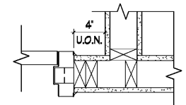
2 TYPICAL DOOR JAMB DIMENSION SCALE: 1/2" = 1'-0"
