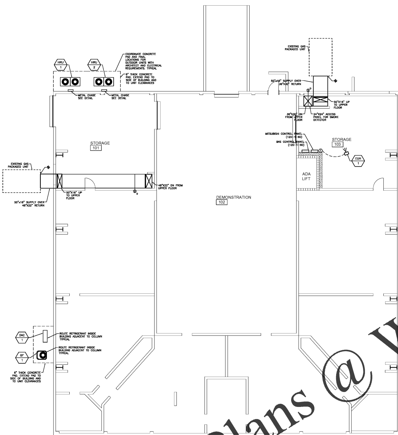
REVISED LOWER FLOOR HVAC PLAN - BASE BID
