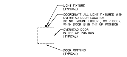
2 TYPICAL UNIT - LIGHTING E3.0 SCALE: NTS
