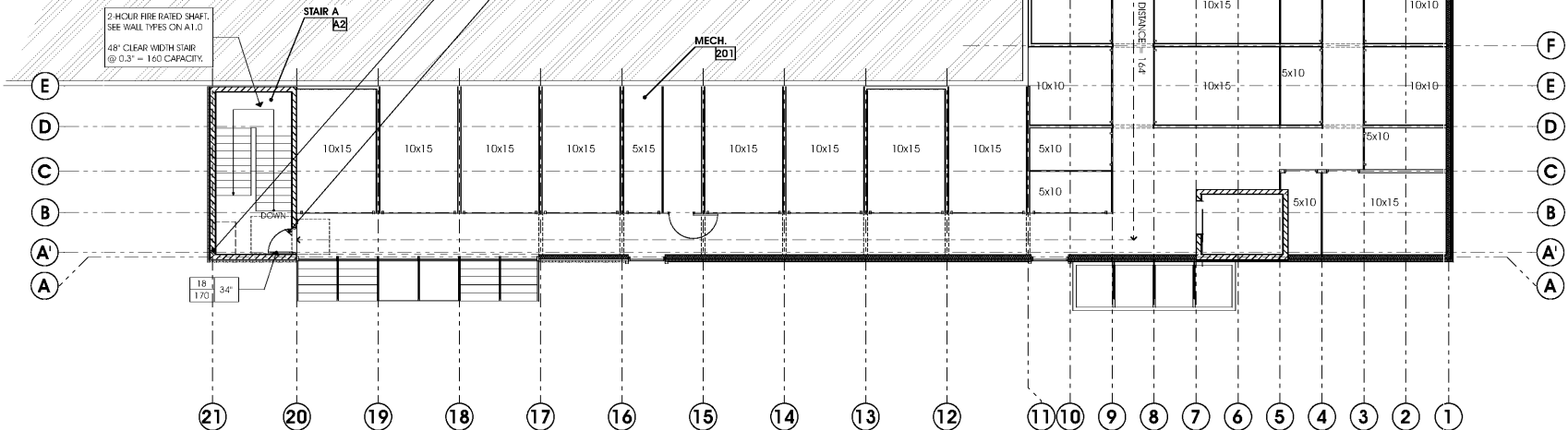
1 EGRESS PLAN SECOND FLOOR SCALE: 1/8"=1'-0"
