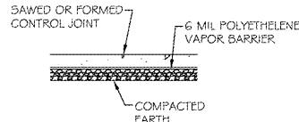
3 CONTROL JOINT DETAIL S01 SCALE: 1/2" = 1'-0"
