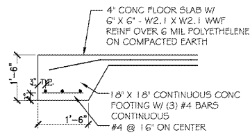
2 TURNED DOWN SLAB DETAIL S01 SCALE: 1/2" = 1'-0"
