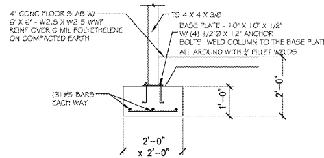
4 COLUMN FOOTING DETAIL S01 SCALE: 1/2" = 1'-0"
