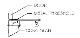
5 THRESHOLD DETAIL SCALE: 1" = 1'-0"
