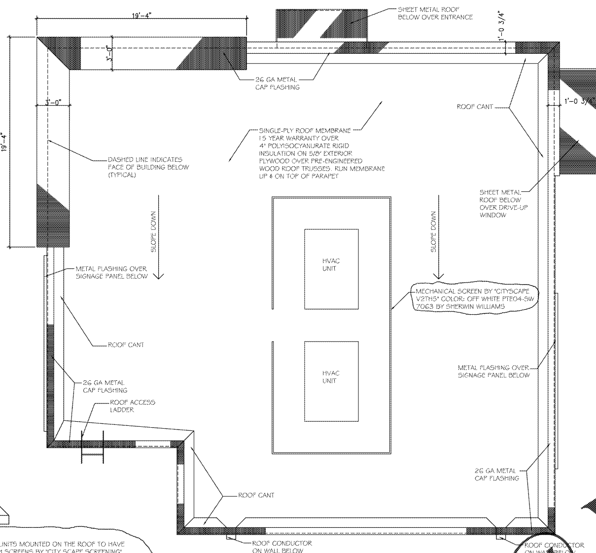
2 ROOF PLAN SCALE: 1/4" = 1'-0"
