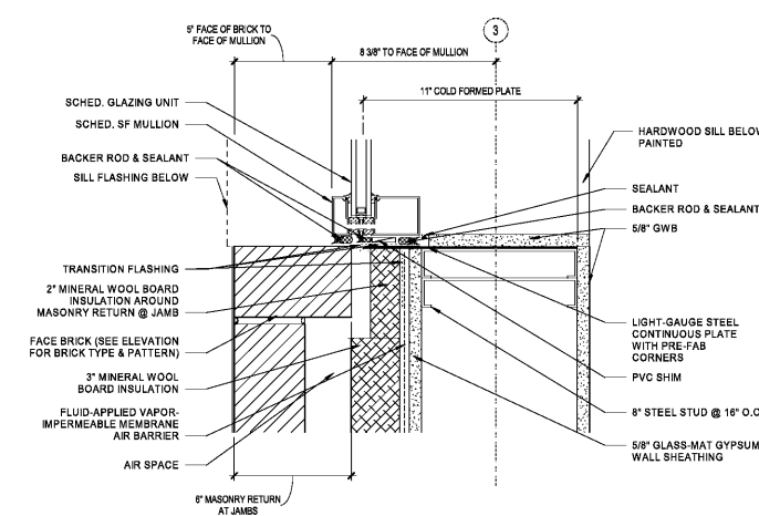
1 PLAN DETAIL - W01 @ SF-1 TYP. AE512 3" = 1'-0" REF 1 / AE101
