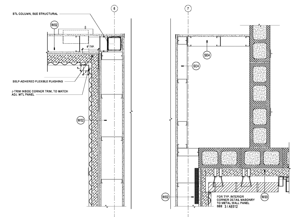
8 PLAN DET. @ CONNECTOR TO NEW ADDITION 1 1/2" = 1'-0"
