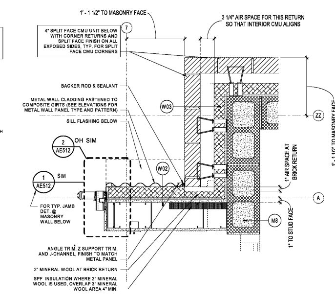
3 PLAN DETAIL - GRID A / 7 AE512 1 1/2" = 1'-0" REF 1 / AE101
