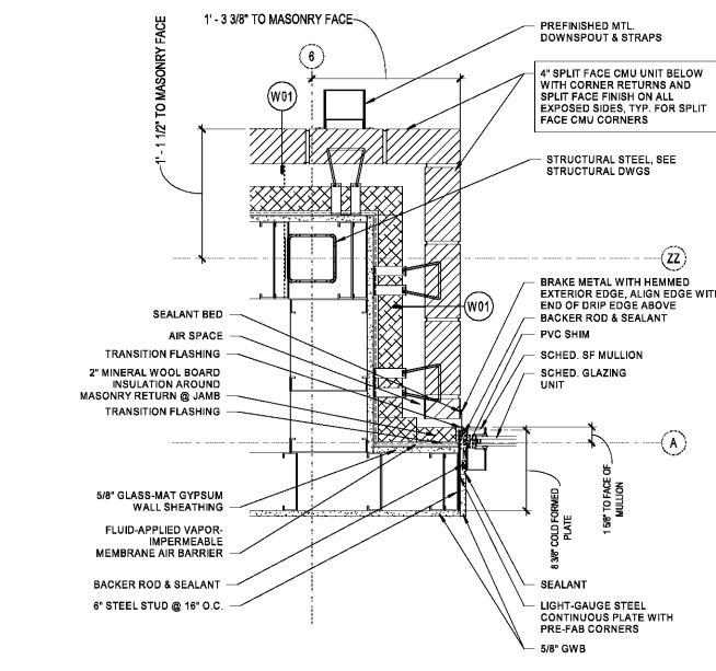
5 PLAN DETAIL - GRID ZZ / 6 AE512 1 1/2" = 1'-0" REF 1 / AE101
