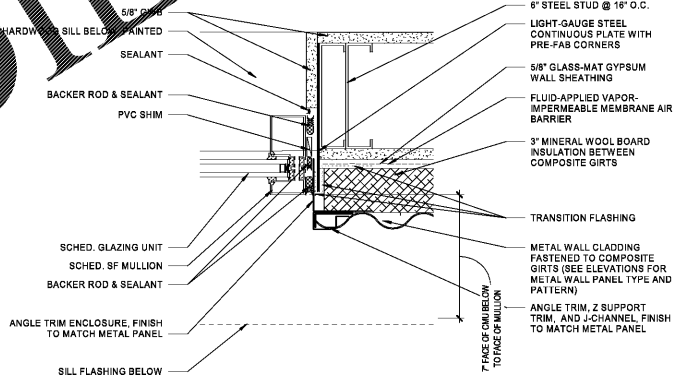
2 PLAN DETAIL - W02* @ SF-1 TYP. AE512 3" = 1'-0" REF 1 / AE101
