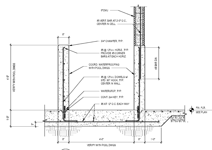
1 BACKWASH TANK SECTION S202 3/4" = 1'-0"
