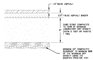
D2.01 TYPICAL HEAVY DUTY PAVEMENT CROSS SECTION NOT TO SCALE
