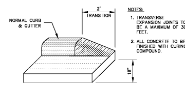
D2.02 CURB & GUTTER END TREATMENT NOT TO SCALE
