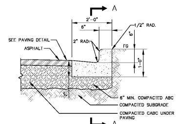
D2.01 TYPICAL HEAVY DUTY PAVEMENT CROSS SECTION NOT TO SCALE
