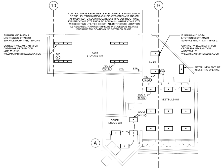
4 GM VESTIBULE LIGHTING PLAN 1/8" = 1'-0"
