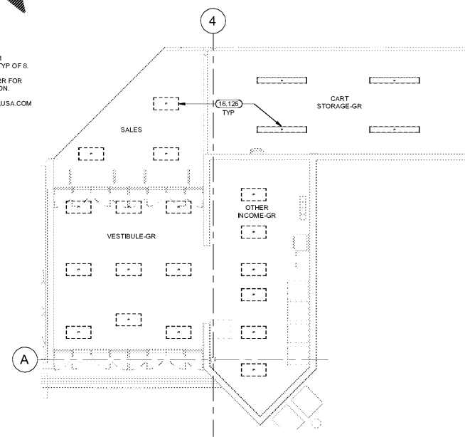
1 GR VESTIBULE LIGHTING DEMO PLAN 1/8" = 1'-0"
