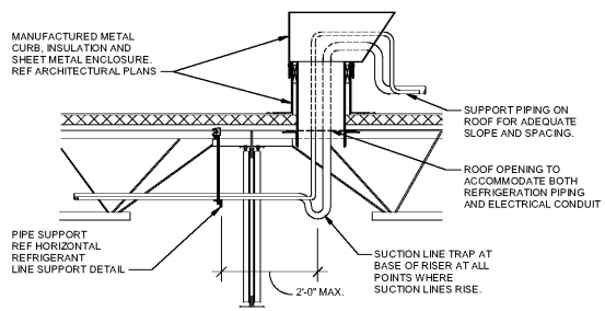
8 ROOF PENETRATION NTS
