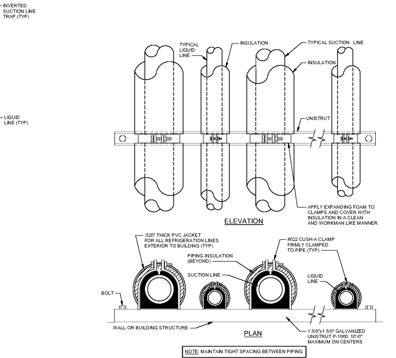
1 VERTICAL REFRIGERANT LINE SUPPORT NTS
