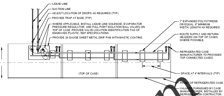
7 REFRIGERATION PIPE ROUTING FOR TOP FEED CASES NTS
