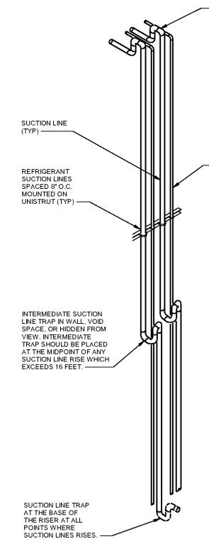
2 INTERMEDIATE SUCTION LINE TRAP NTS
