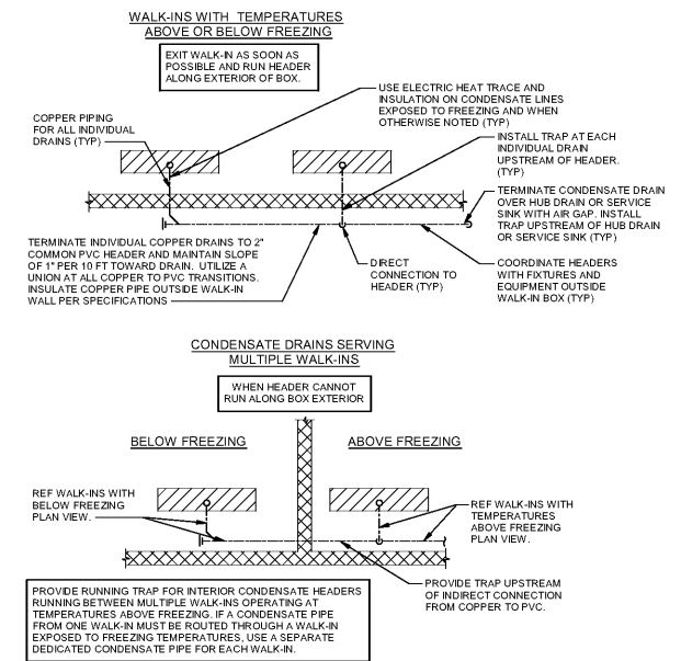
6 EVAPORATOR COIL CONDENSATE PIPING NTS
