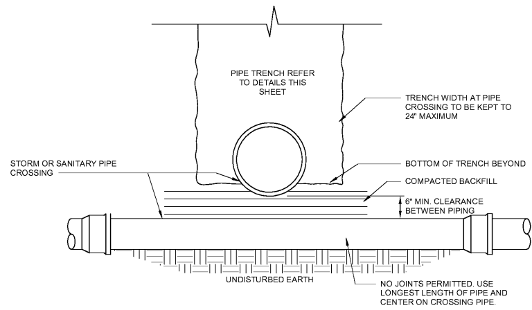
4 DETAIL - UNDERGROUND PIPE CROSSING P3.2 N.T.S.
