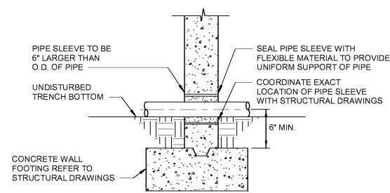
6 DETAIL - FOUNDATION WALL PIPE SLEEVE P3.2 N.T.S.
