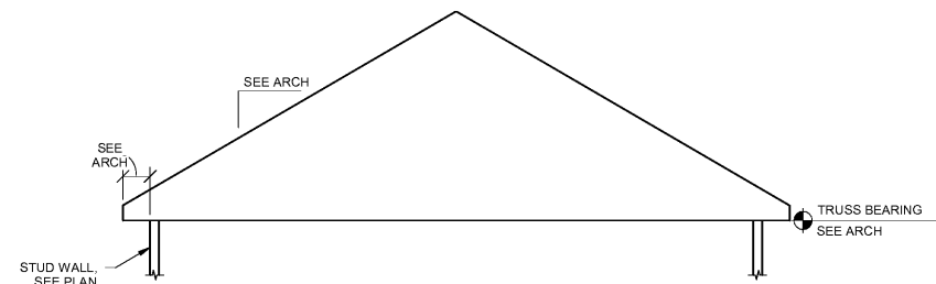
1 TRUSS 3B S6.4 3/16" = 1'-0"
