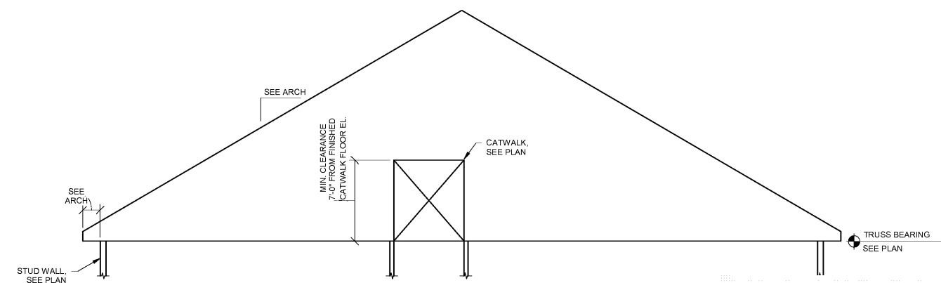
5 TRUSS 2 S6.3 3/16" = 1'-0"
