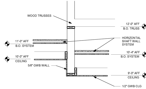
2 SOFFIT DETAIL @ CORRIDOR A1.5 3/4" = 1'-0"
