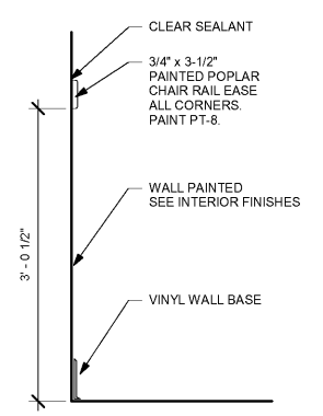
4 CHAIR RAIL @ CORRIDOR A1.4 1" = 1'-0"
