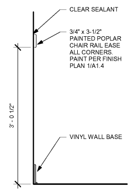
3 CHAIR RAIL @ CLASSROOMS A1.4 1" = 1'-0"
