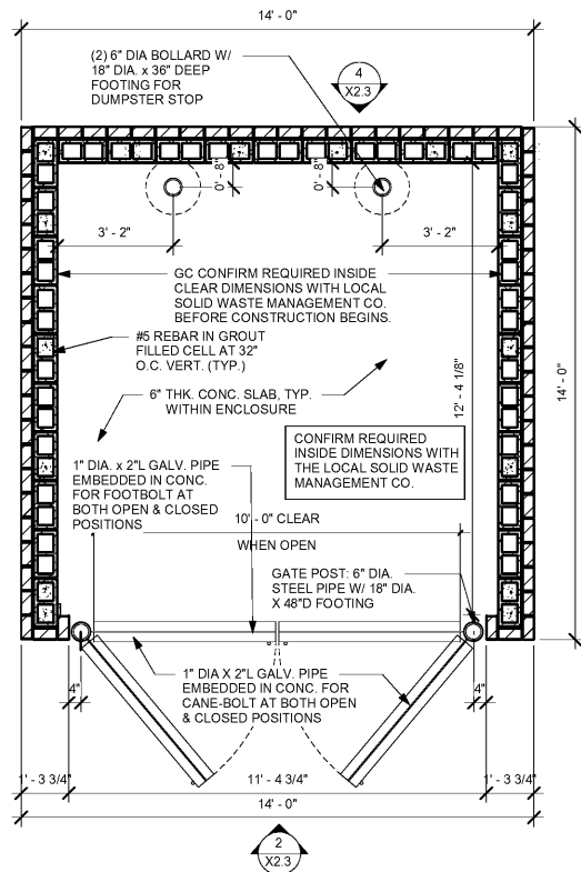
1 TRASH ENCLOSURE PLAN X2.3 3/8" = 1'-0"
