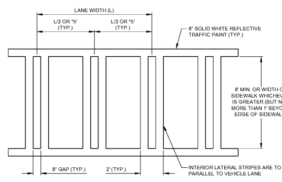
CROSSWALK STRIPING NOT TO SCALE
