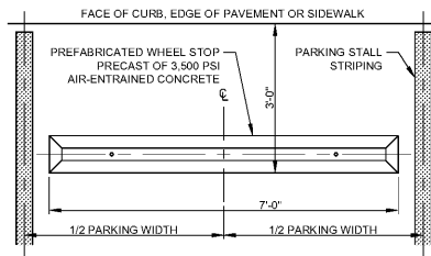
CONCRETE WHEEL STOP NOT TO SCALE
