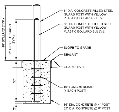
BOLLARD NOT TO SCALE
