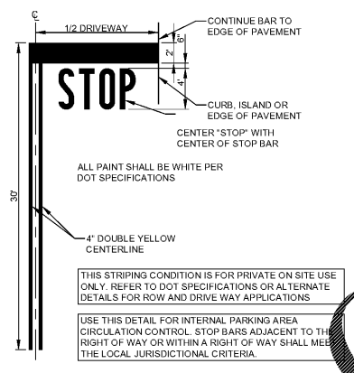
STOP BAR AND LABEL STRIPING NOT TO SCALE
