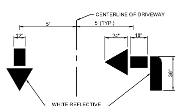
DRIVEWAY TRAFFIC FLOW DIRECTIONAL ARROW NOT TO SCALE
