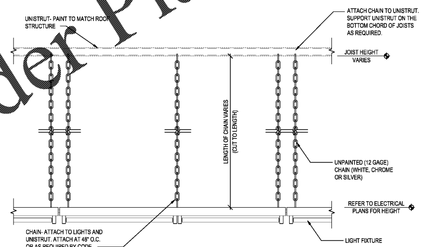
1 LIGHT MOUNTING DETAIL "OPEN CEILING" SCALE: NTS
