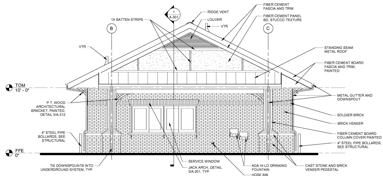
1 BUILDING ELEVATION - NORTH WEST
