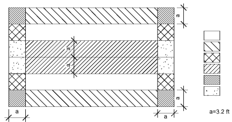
WIND ZONE DIAGRAM MAIN
