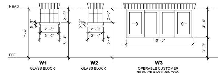
WINDOW TYPES SCALE: 1/4" = 1'-0"
