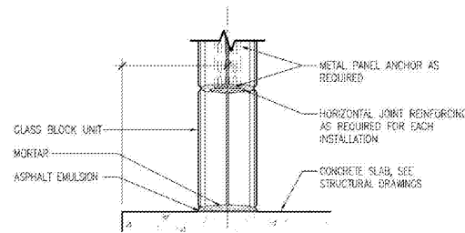
2 GLASS BLOCK DETAIL SCALE: 1/2" = 1'-0"
