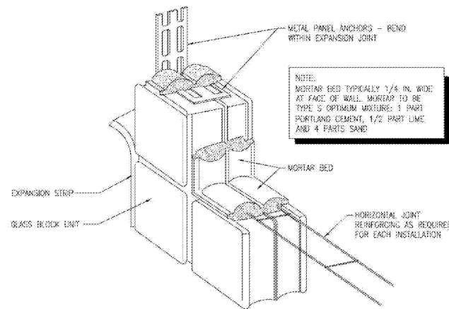
1 GLASS BLOCK DETAIL NTS
