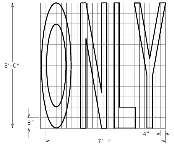
TYPE 1 AREA = 20.8 FT 2
