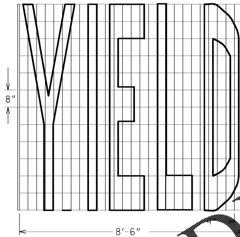
TYPE 15 AREA = 25.4 FT 2
