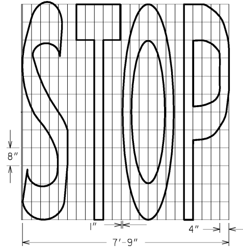
TYPE 2 AREA = 25.4 FT 2
