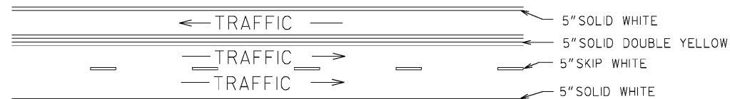
TWO-WAY TRAFFIC WHERE MOTORISTS IN A SINGLE LANE ARE NOT PERMITTED TO PASS
