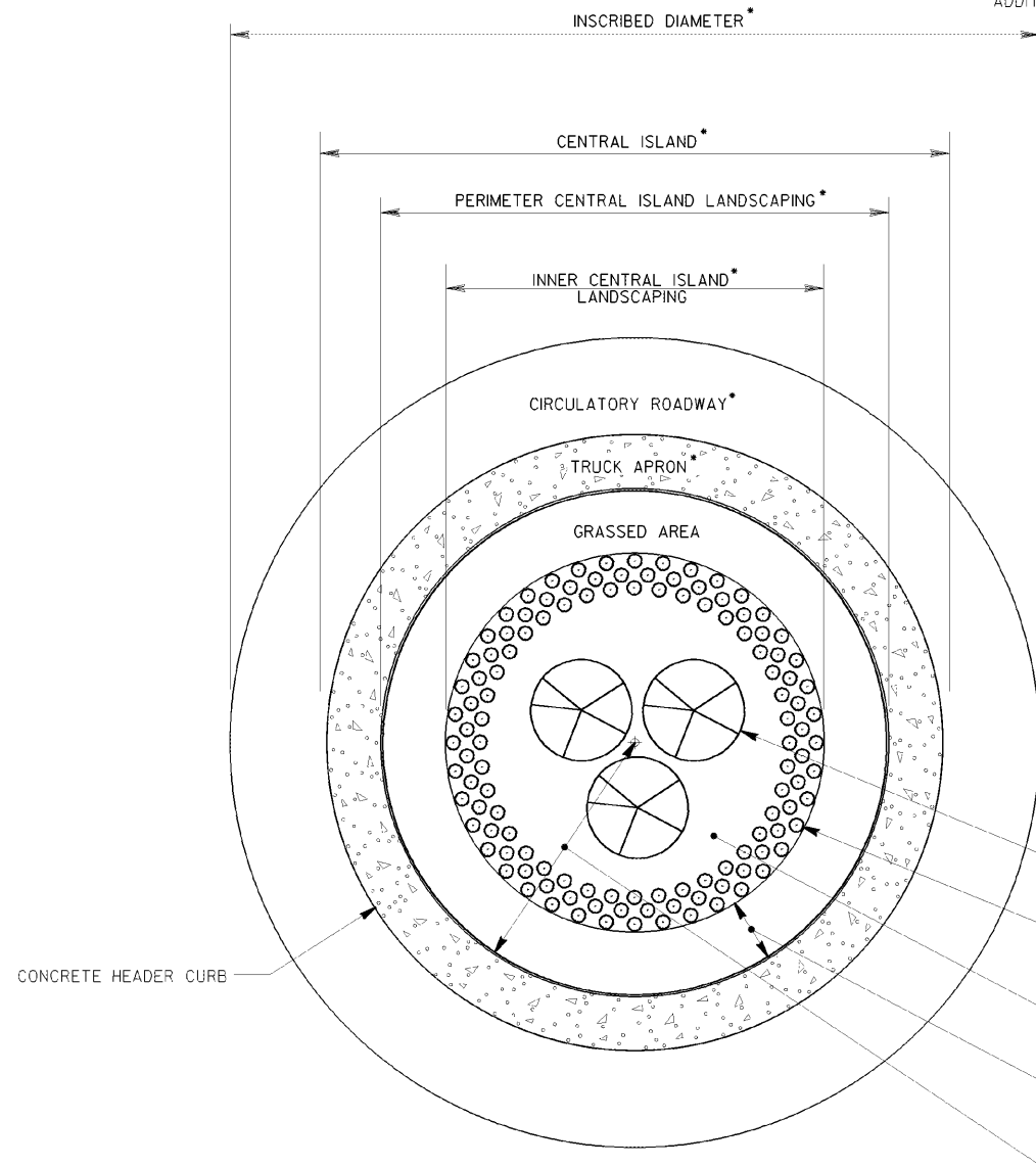
PLANTING LAYOUT NO SCALE
