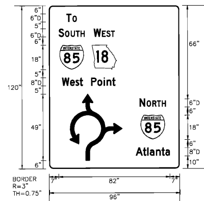
D1-5 - #2 GREEN BACKGROUND WITH WHITE TEXT STA. 28+20, SR 18 WB SHDLR 1 EACH REQ'D
