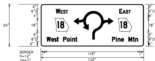
D1-5 - #131 GREEN BACKGROUND WITH WHITE TEXT STA. 199+98, SR 103 NB SHDLR 1 EACH REQ'D
