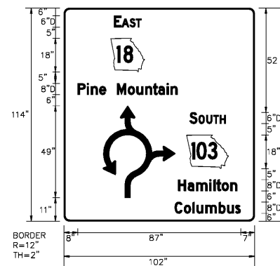
D1-5 - #3 GREEN BACKGROUND WITH WHITE TEXT STA. 39+20, SR 18 EB SHDLR 1 EACH REQ'D
