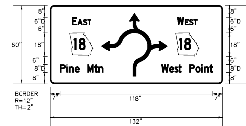
D1-5 - #132 GREEN BACKGROUND WITH WHITE TEXT STA. 406+79, SB EXIT RAMP 1 EACH REQ'D
