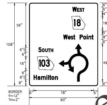
D1-5 - #4 GREEN BACKGROUND WITH WHITE TEXT STA. 51+72, SR 18 WB SHDLR 1 EACH REQ'D
