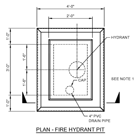
PLAN - FIRE HYDRANT PIT
