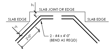
Short Slab Extension
