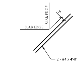
Re-entrant Corner
