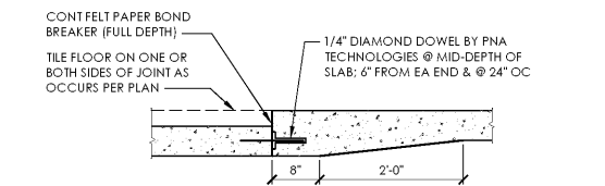
Construction Joint @ Concrete Step
