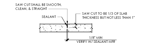
Control Joint
