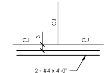
Discontinuous Control Joint
