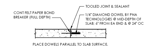
Construction Joint
