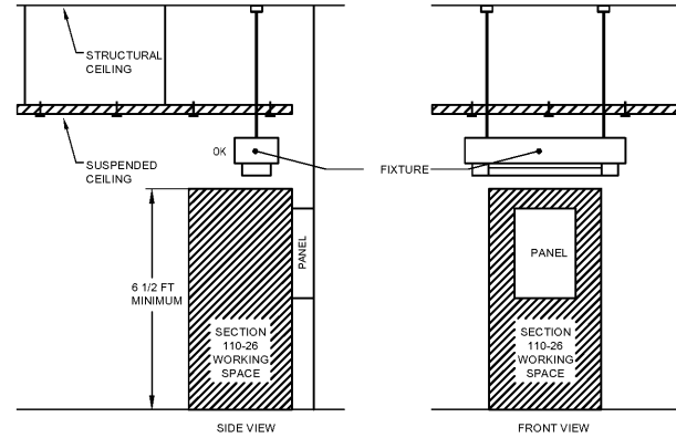
2 WORKING CLEARANCE FOR ELECTRICAL EQUIPMENT
