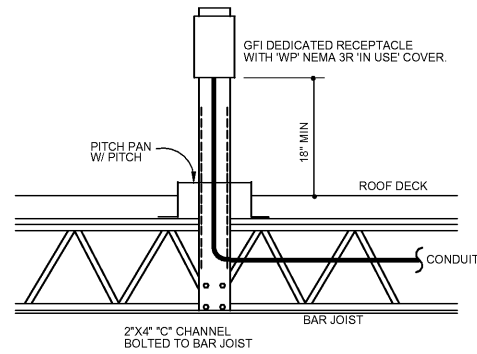
1 ROOFTOP RECEPTACLE DETAIL
