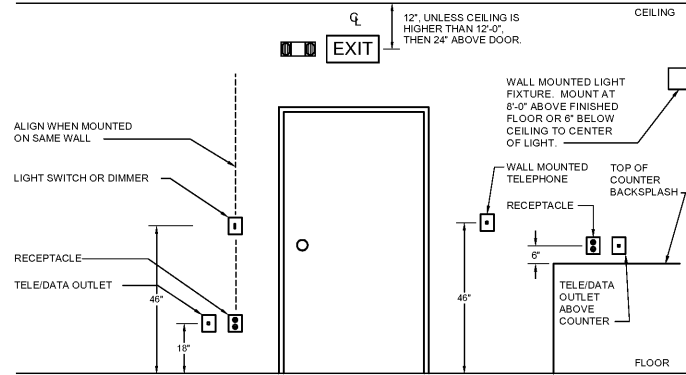
4 DEVICE MOUNTING ELEVATION
