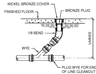
2 FLOOR CLEANOUT DETAIL P2.01 NOT TO SCALE
