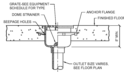
1 FLOOR SINK DETAIL P2.01 NOT TO SCALE
