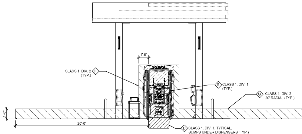
3 END ELEVATION 1/4" = 1'-0"
