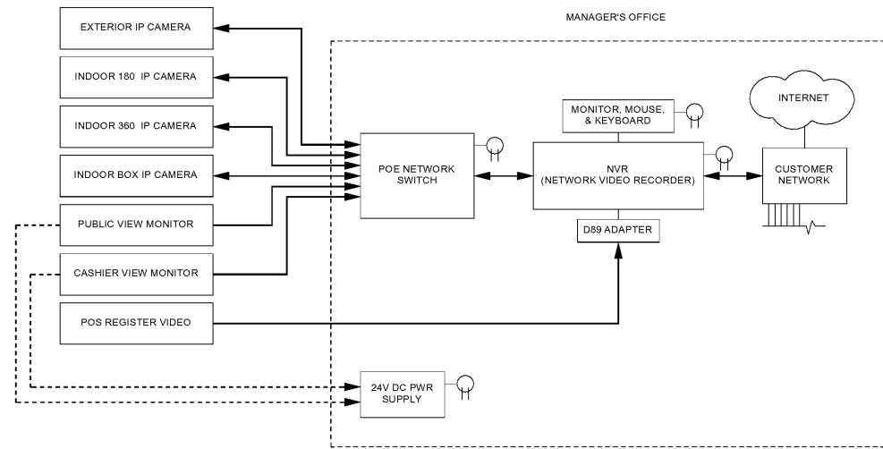
3 STANDARD 7-ELEVEN IP CCTV TOPOLOGY N.T.S.
