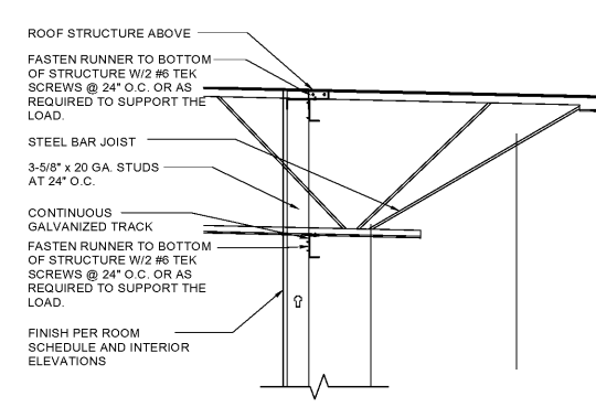
1 TYP. PARTITION TO DECK DETAIL 3/4" = 1'-0"
