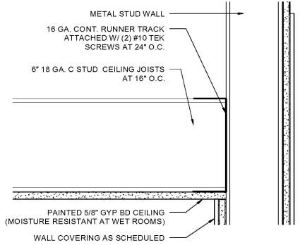
2 CEILING DETAIL 3" = 1'-0"
