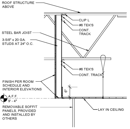
3 SECTION @ BULKHEAD 3/4" = 1'-0"
