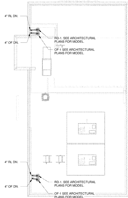
3 P1.1 1/8" = 1'-0" PLUMBING ROOF PLAN
