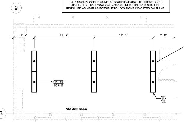
2 GM VESTIBULE LIGHTING PLAN 1/4" = 1'-0"
