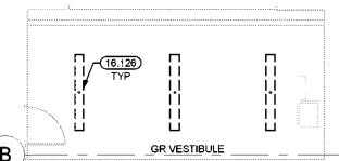
3 GR VESTIBULE LIGHTING DEMO PLAN 1/8" = 1'-0"
