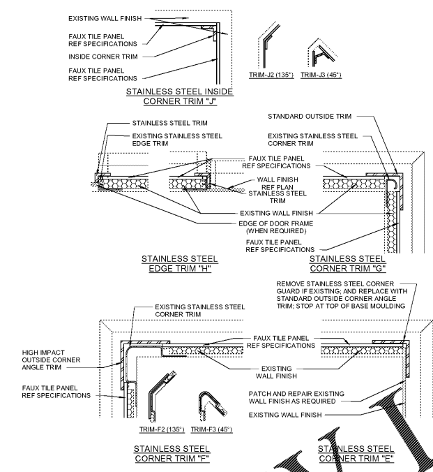
② CORNER GUARD AND TRIM 6" = 1'-0"
