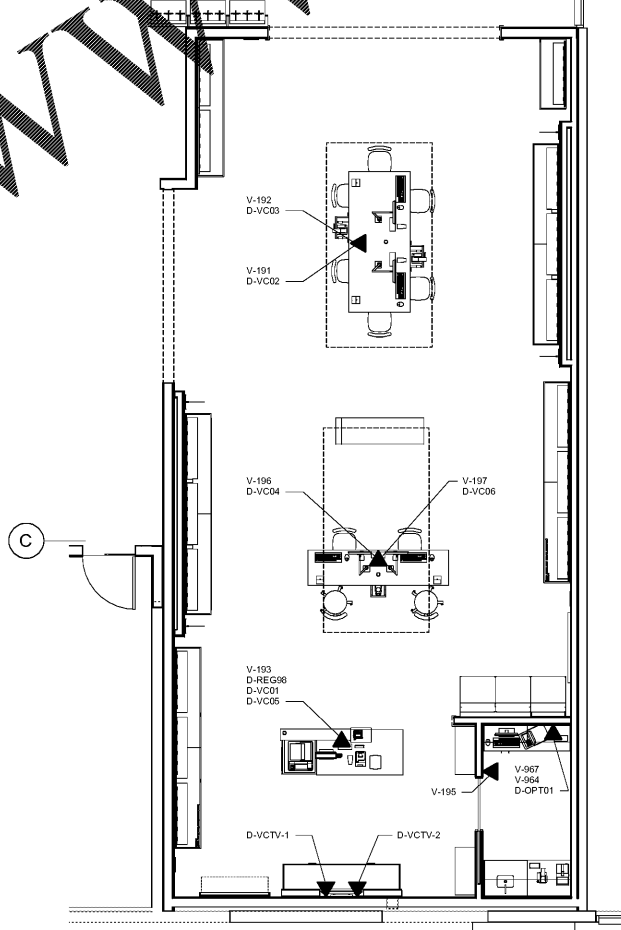
2 VISION CENTER VOICE / DATA PLAN 1/4" = 1'-0"
