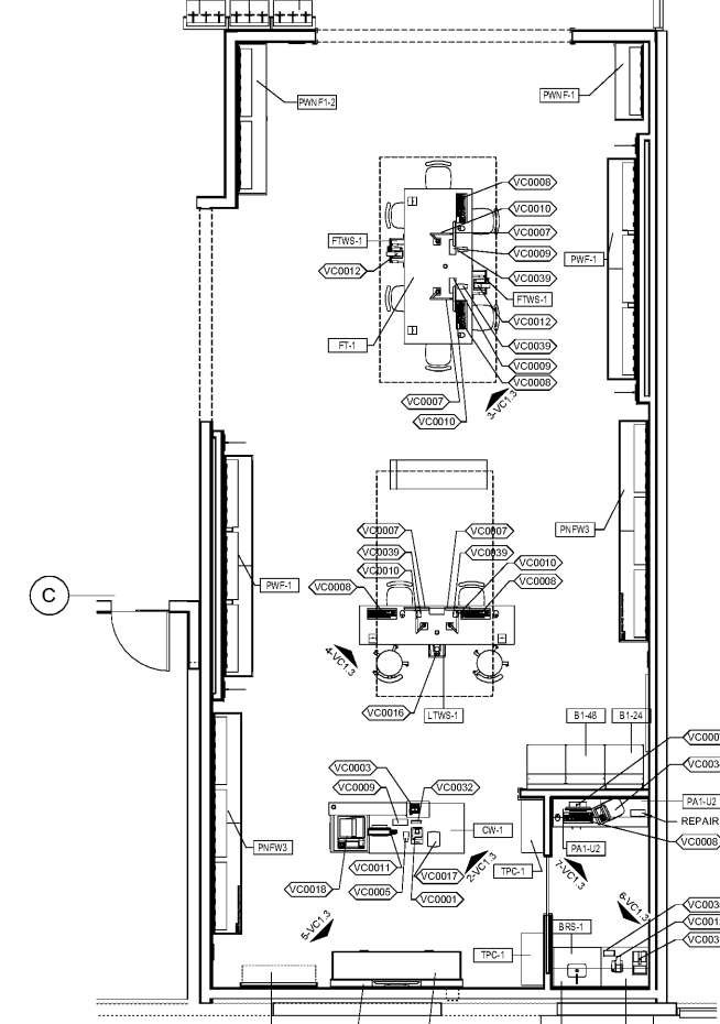
1 VISION CENTER EQUIPMENT PLAN 1/4" = 1'-0"
