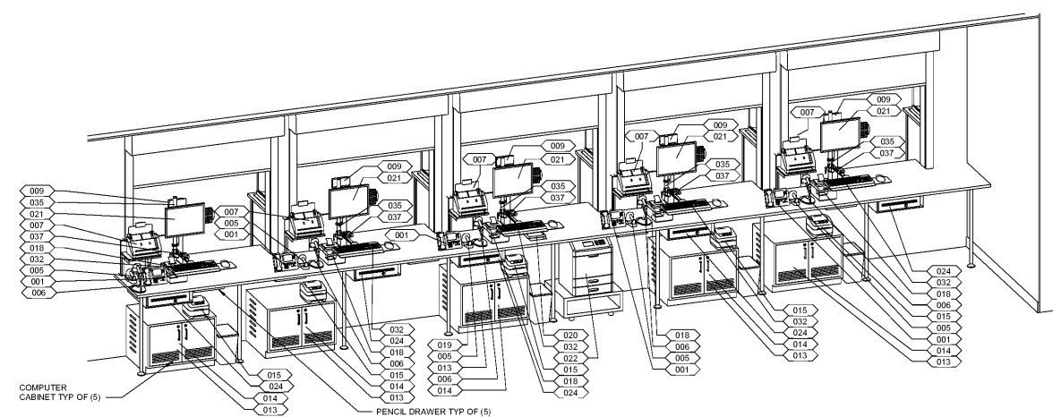
1 SERVICE COUNTER EQUIPMENT 1/2" = 1'-0"
