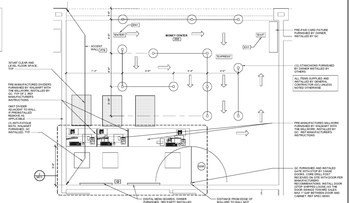
1 MONEY CENTER PLAN 3/8" = 1'-0"
